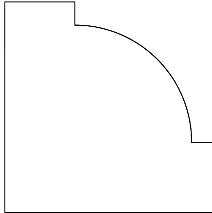
#269780 2-1/4" x 2-1/4"/1.25" rad
