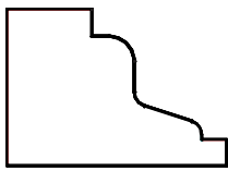
#200160 3/4" x 1-1/8"
