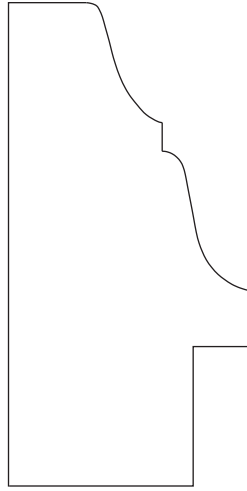
#59165 1" x 2-1/2"
