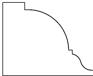
#141350 1-1/4" x 1-9/16"
