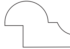
PF-42 1-1/8" x 13/16"
