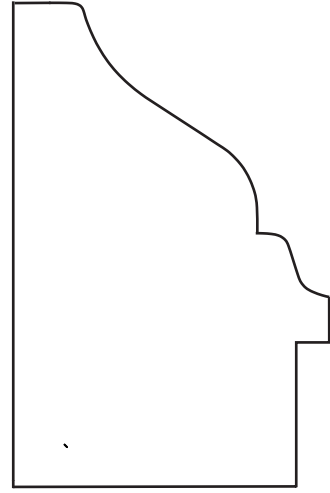
#82745 1-1/2" x 2-1/2"
