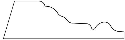
#169380/85 3/4" x 2-7/16"
