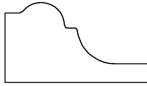
#3311140 (108735) 7/8" x 1-1/2"
