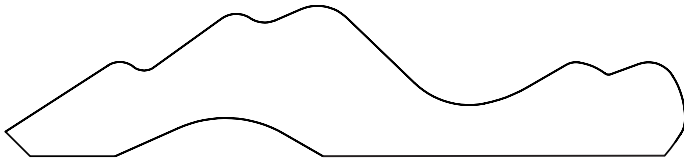
#71450/55/60/65 3/4" x 3-1/2"
